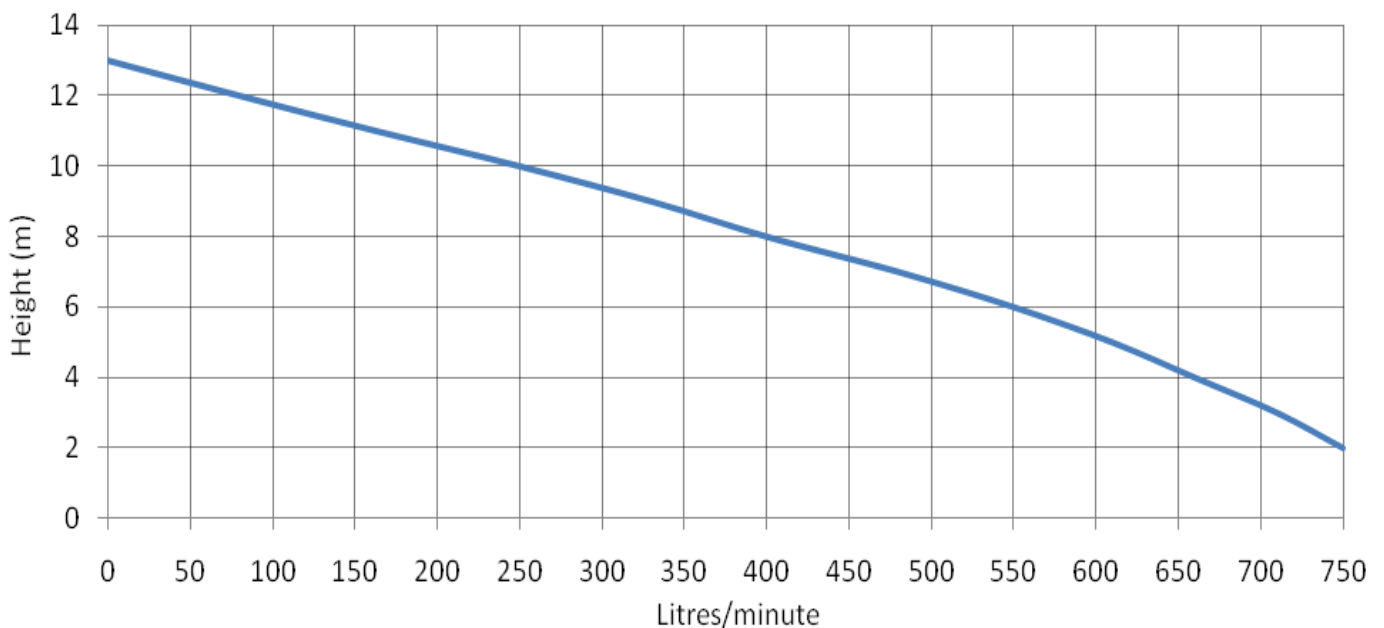
Pump Performance
